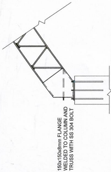
DETAIL -A NTS
