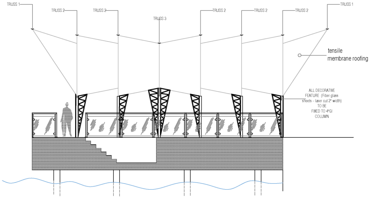
Decorative Feature Detail
