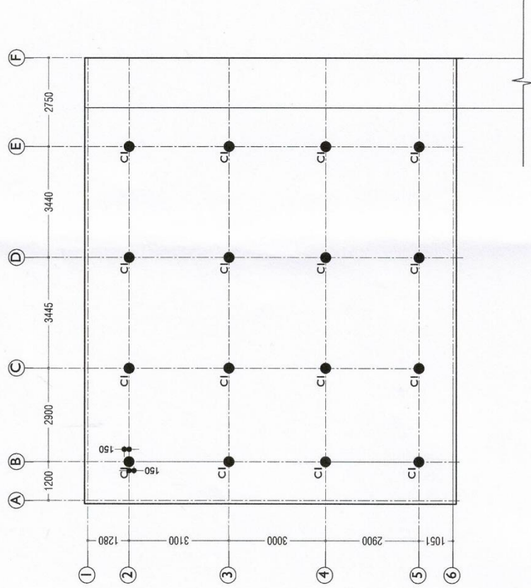
COLUMN LAYOUT BELOW DECK SCALE : 1/100
